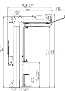
Cobra RA Cobra Rotary Arm with integrated control panel
