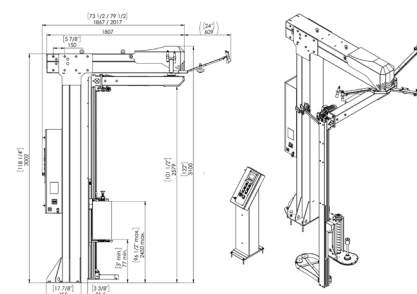
Cobra RA Cobra Rotary Arm with stand-alone control panel
