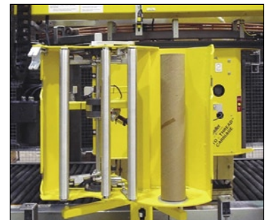
With the new film roll in ready position, the Auto Roll Changer returns to its home position. Wrapping resumes and film can be replenished at the operator's convenience.
