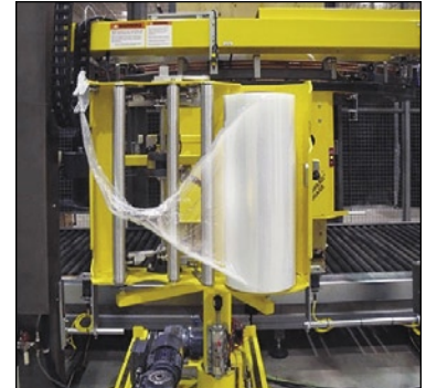
Auto Roll Changer, with new roll of film, in home position.
